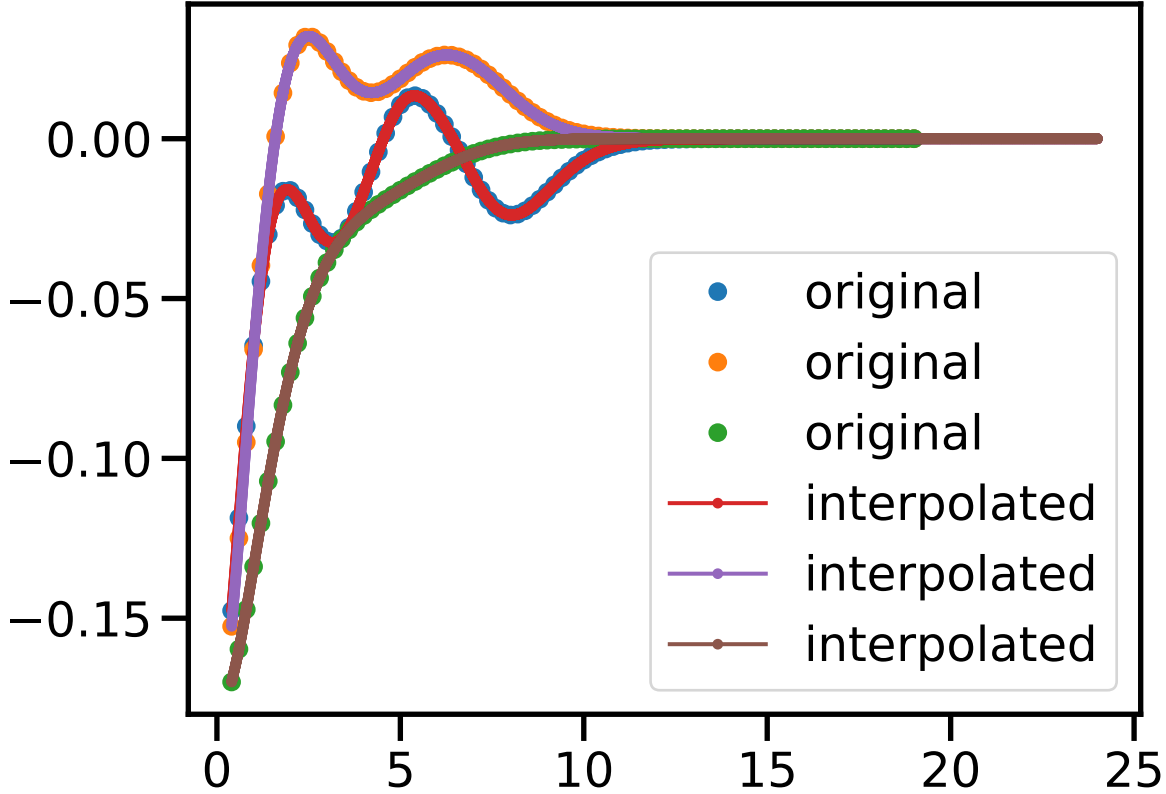
Hamiltonian Interpolation Before Training (14, 14, 2, 2)
